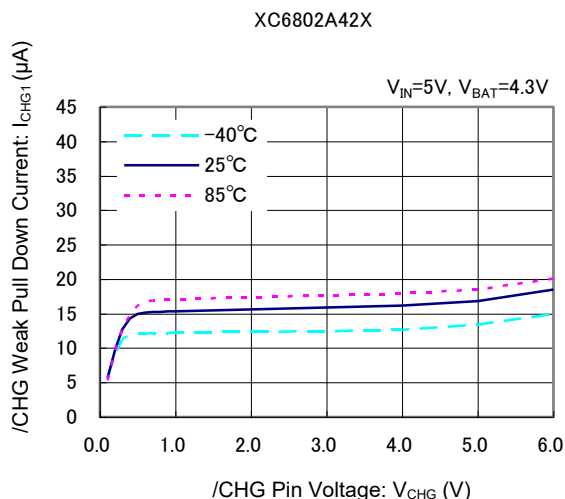
(18) /CHG Weak Pull Down Current vs. /CHG Pin Voltage
