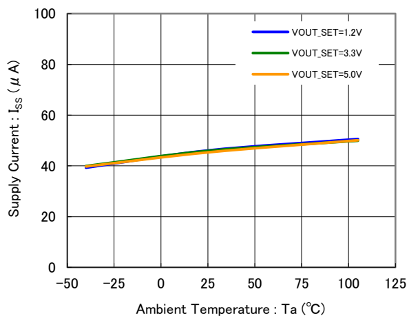
XC6230
