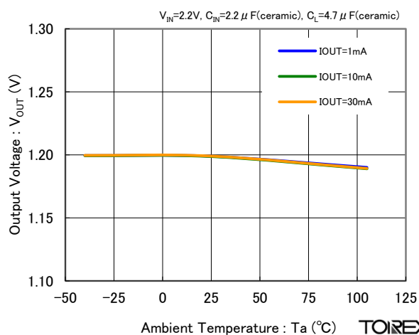
XC6230( V_{OUT,SET}=1.2V )
