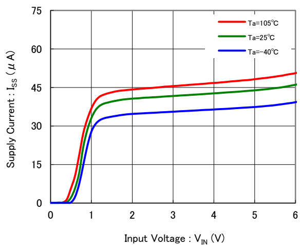
XC6230( V_{OUT,SET}=1.2V )
