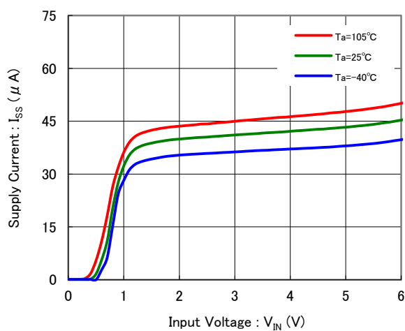
XC6230( V_{OUT,SET}=3.3V )
