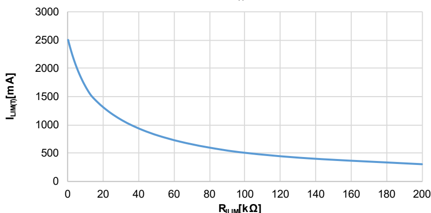
XC6230 Current Limit(I LIM(T) ) vs External Resistor(R LIM )
