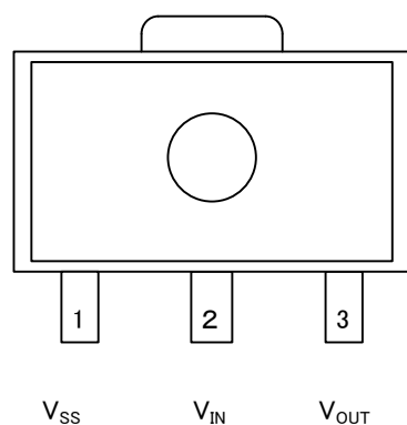
SOT-89 (TOP VIEW)
