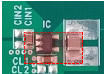
Stand-alone DC/DC External parts : 3 pcs
